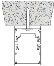
Solid Ceiling 1/4"-20 Thread Required (1)
