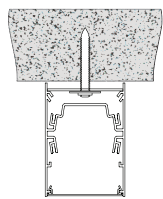
Solid Ceiling 1/4"-20 Thread Required (1)
