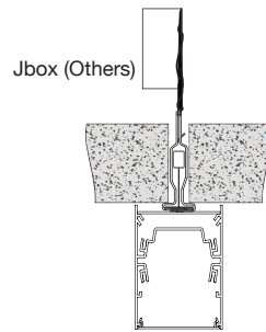
T-Bar 15/16" Aircraft Cable (ACY)
