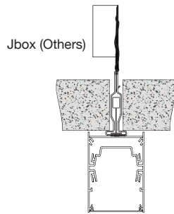
T-Bar 9/16" Aircraft Cable (ACY)
