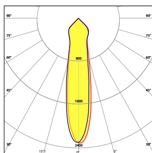
20° Spot Beam
