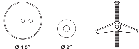
Aircraft Cable Canopy / Drywall Anchor
